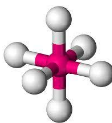
(L) Alfred Werner (R) Octahedral configuration
